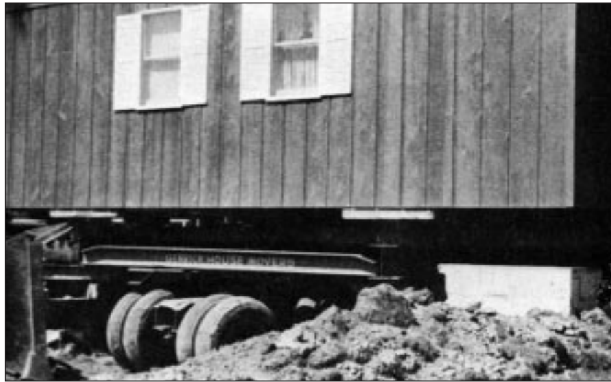
Figure 7-2 Trailer wheel sets are placed beneath the lifting beams.
